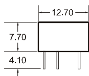
BXXXXD-1W Package
