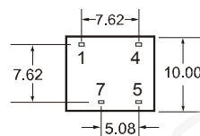
BXXXXD-1W Footprint
