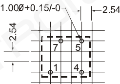
BXXXXD-1W Footprint
