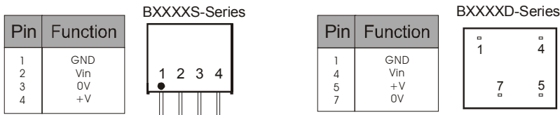
BXXXXS-1W Package
