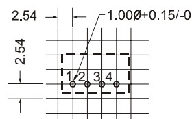
BXXXXS-1W Footprint
