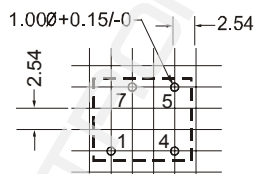
BXXXXD-1W Footprint
