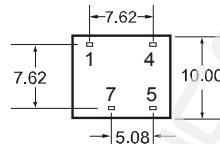
BXXXXD-1W Footprint
