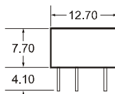
BXXXXD-1W Package
