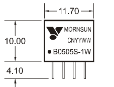
BXXXXS-1W Package
