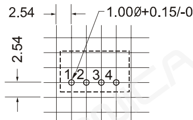
FXXXXM-1W Footprint
