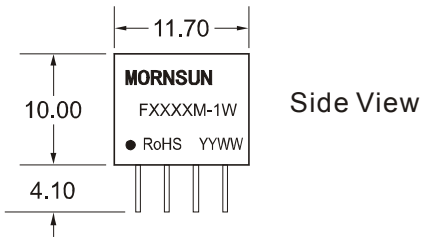
FXXXXM-1W Package
