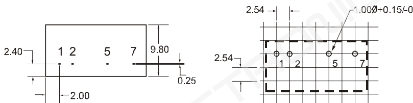
Bottom View
