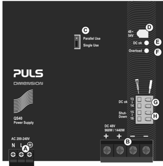
Fig. 14-1 Front side
