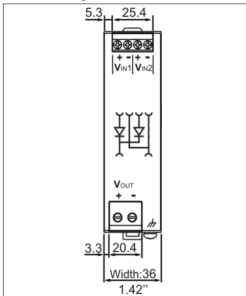
Fig. 17-1 Front view
