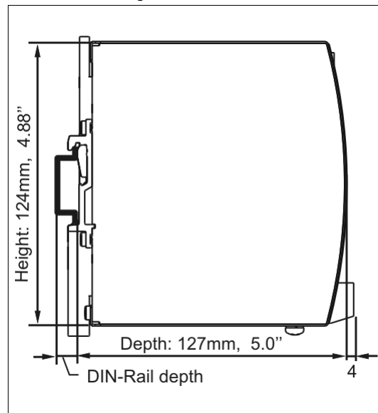
Fig. 17-2 Side view
