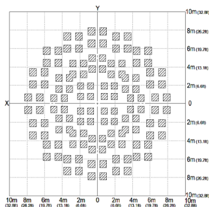
Detection zones distribution on the ground (@12m mounting height)
