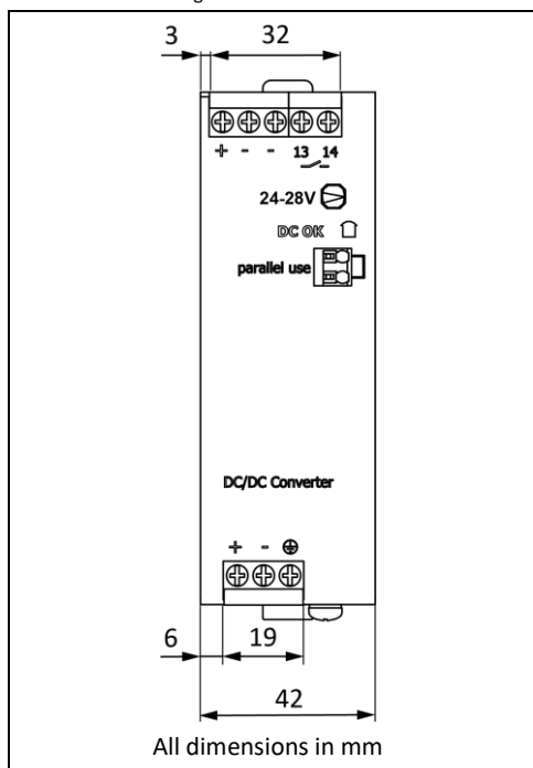
Fig. 21-1 Front view
