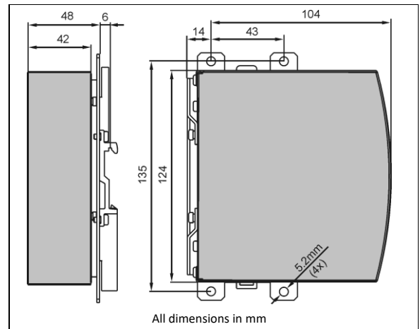
Fig. 22-9 Hole pattern
