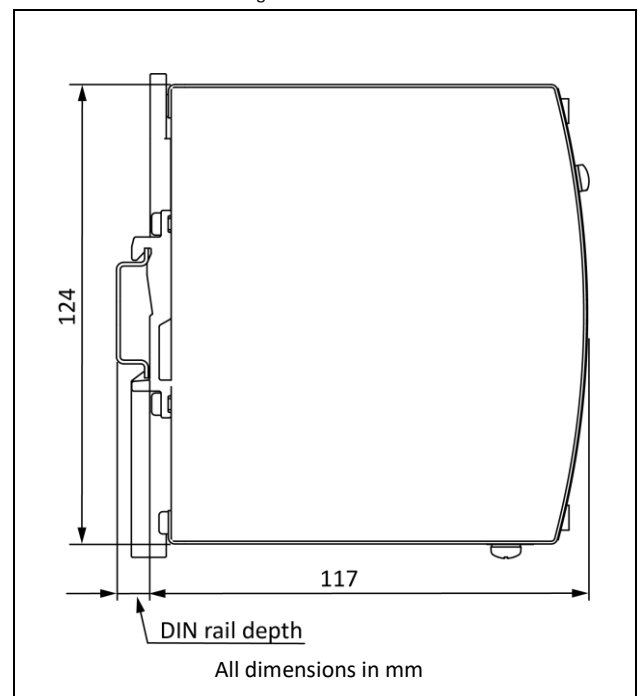
Fig. 21-2 Side view
