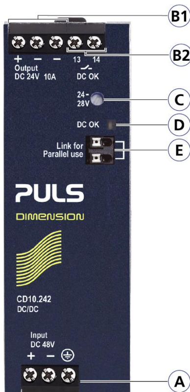
Fig. 11-1 Front side
