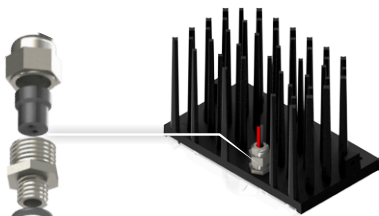
(CoolBlock® cross-section)
