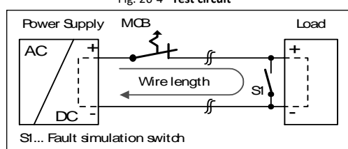
Fig. 26-4 Test circuit
