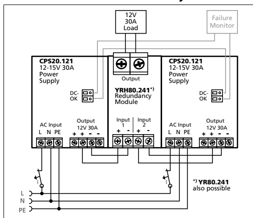
Fig. 22-1 Typical 1+1 Redundant configuration for 30A with a dual redundancy module
