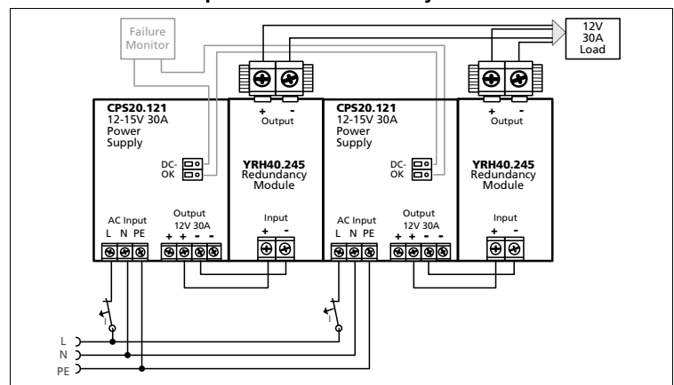
Fig. 22-2 Typical N+1 or 1+1 Redundant configuration for 30A with multiple YRH40.245 redundancy modules
