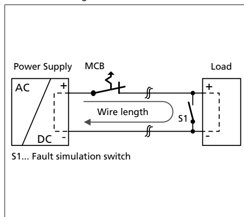
Fig. 23-3 Test circuit
