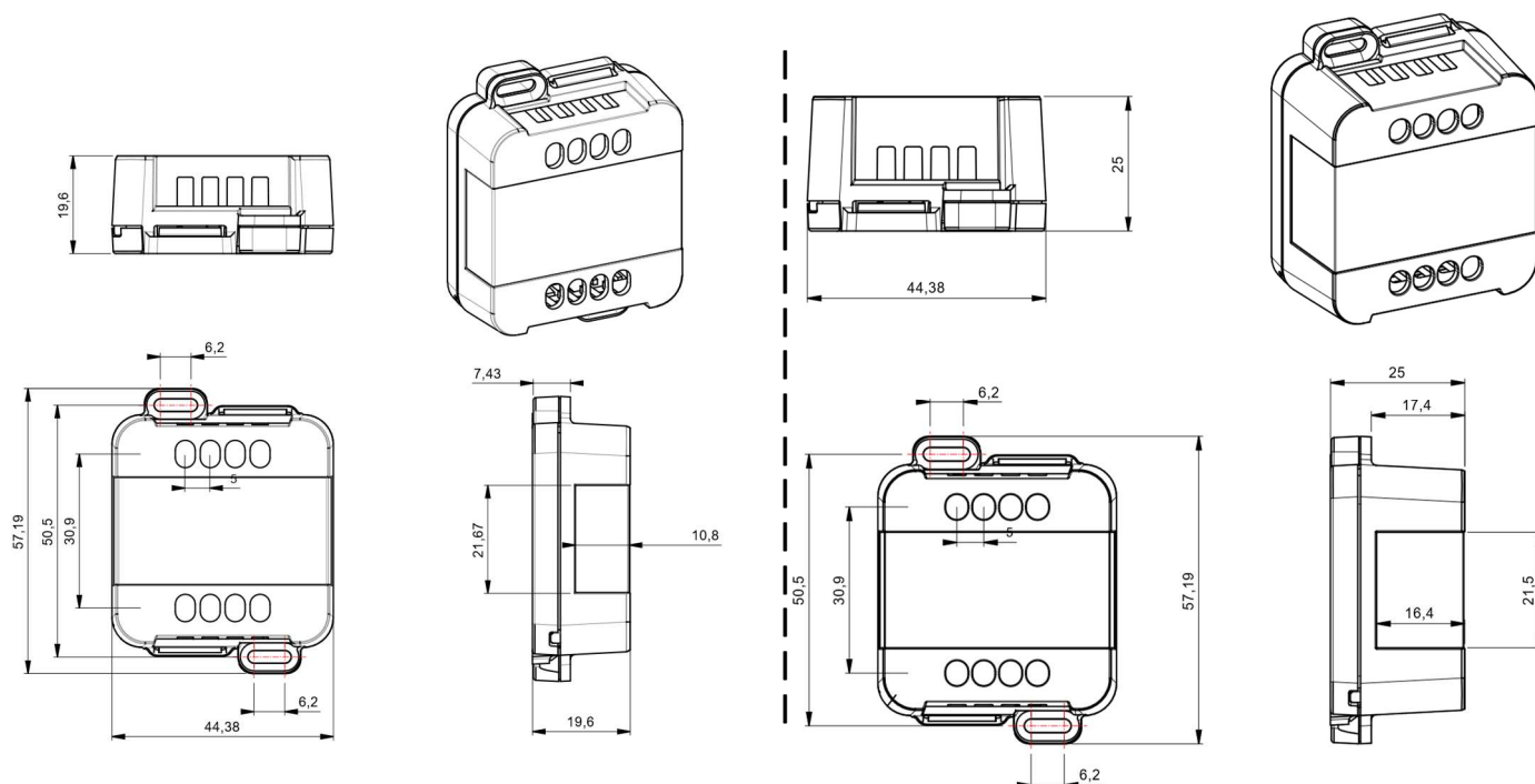
DLM1224-1CV-BUS Variant
