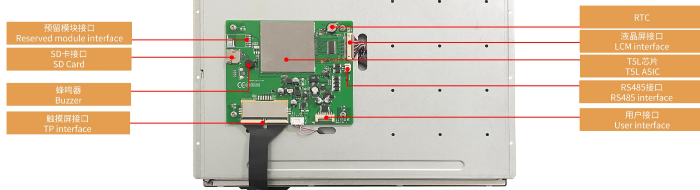
硬件接口图 Hardware interface
