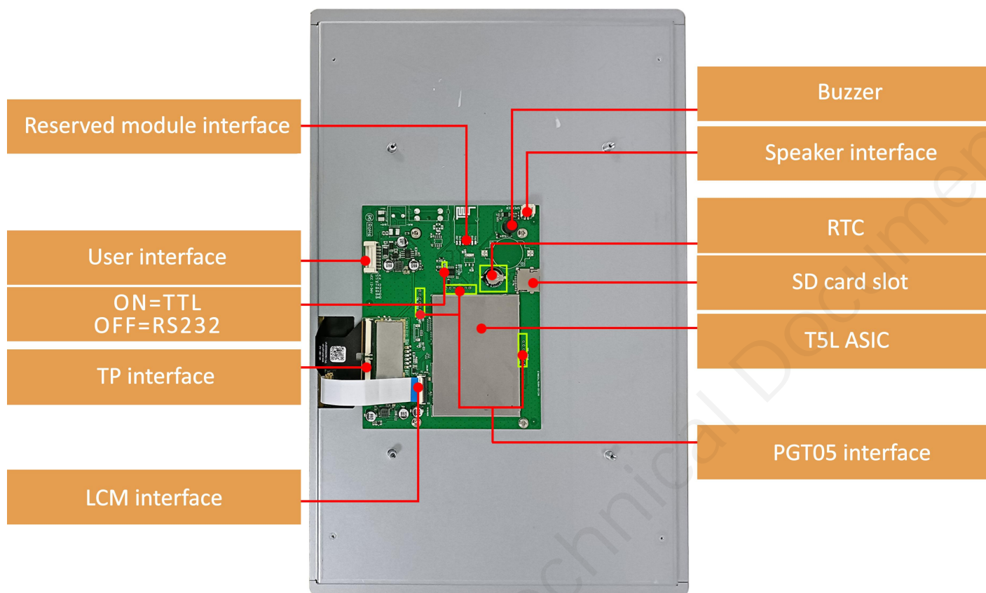
Hardware interface
