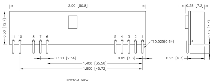
BOTTOM VIEW
