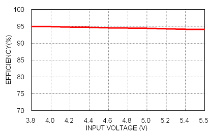
DOS16-05T, Vout=3.3V Efficiency vs. Input Voltage
