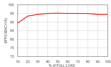
DOS16-05T, Vout=3.3V Efficiency vs. Output Load
