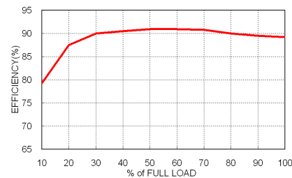
DOS06-12T, Vout=3.3V Efficiency vs. Output Load
