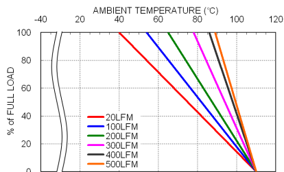
FEC60-48S05 Derating Curve
