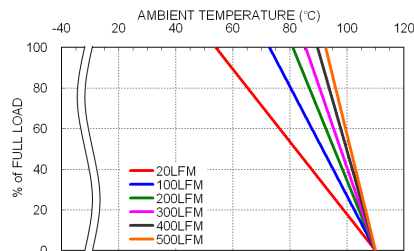
FEC60-48S05 Derating Curve With Heat-sink
