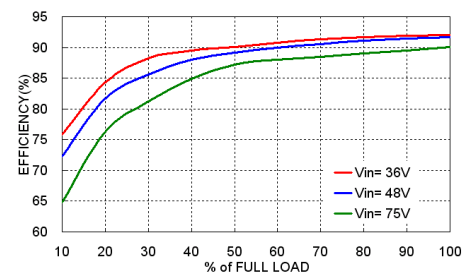
FED40-48S05 Efficiency VS Output Load
