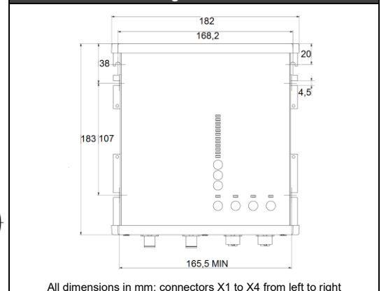
All dimensions in mm; connectors X1 to X4 from left to right
