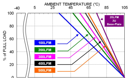
HAE200-72S12UA Derating Curve (See Thermal Considerations)
