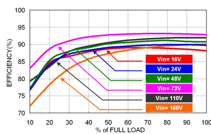
HAE200-72S12UA Efficiency vs. Output Load
