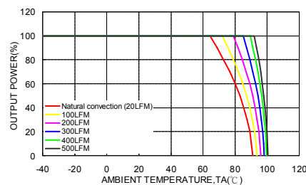
HAE75-48S05W Derating Curve With 0.45" Height Heat-sink (See Thermal Considerations)
