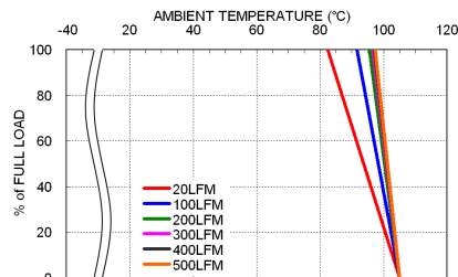
LCD10-48S05 Derating Curve With Heat-sink
