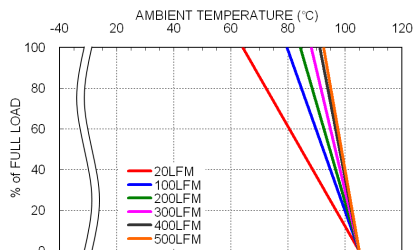
LCD15-48S05W Derating Curve
