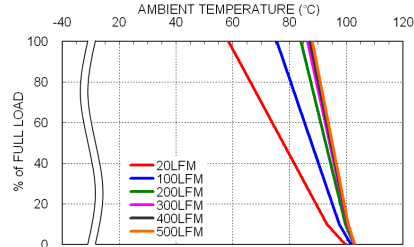
LCD30-48S05 Derating Curve With Heat-sink
