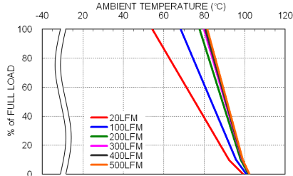
LCD30-48S05 Derating Curve
