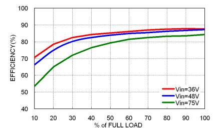
LED15-48S05 Efficiency vs. Output Load
