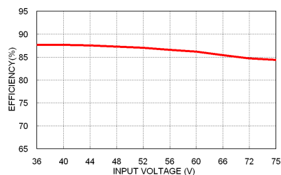
LED15-48S05 Efficiency vs. Input Voltage
