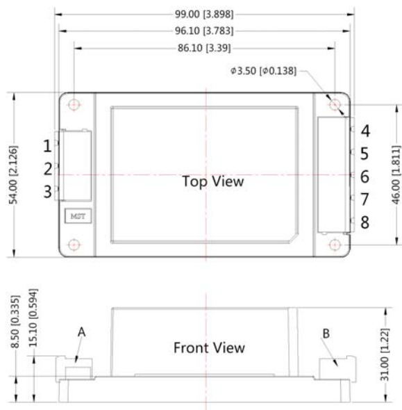
Outline and dimensions (Unit: mm)
