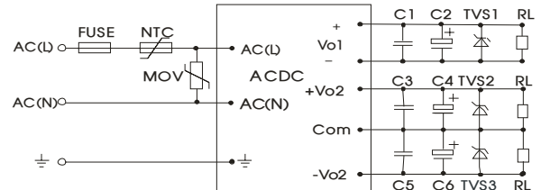
Fig. 4: LHxx-10Cxx(Triple Output) series typical application circuit
