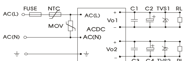
Fig. 3: LHxx-10Dxx(Isolate Twin Output) series typical application circuit
