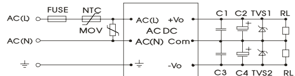
Fig. 2: LHxx-10Axx (Dual Output) series typical application circuit
