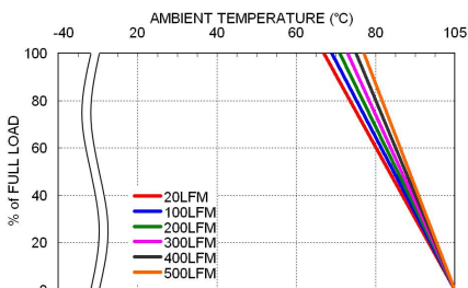
LSR01-12S05 Derating Curve
