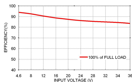
LSR01-12S05 Efficiency vs. Input Voltage
