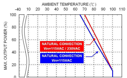
Derating Curve vs. Ambient Temperature MAC15USxxB xx=24/28/36/48/53 Connector Option : (-M / -T / -D)
