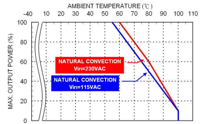
Derating Curve vs. Ambient Temperature MAC15USxxB xx=3P3/05/7P5/09/12/15/18 Connector Option : (-M / -T / -D)
