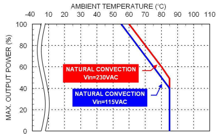
Derating Curve vs. Ambient Temperature MAC15USxxB xx=3P3/05/7P5/09/12/15/18 Connector Option : (Blank: JST)
