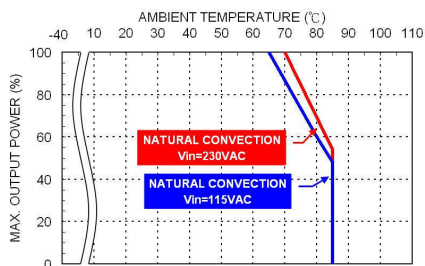
Derating Curve vs. Ambient Temperature MAC15USxxB xx=24/28/36/48/53 Connector Option : (Blank: JST)
