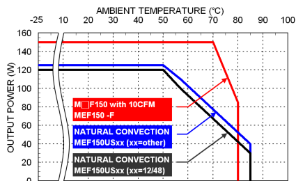
Derating Curve vs. Ambient Temperature V_{in}=115\text{VAC}
