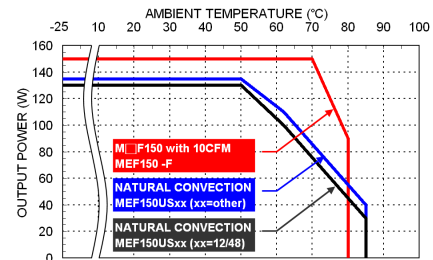
Derating Curve vs. Ambient Temperature V_{in}=230\text{VAC}
