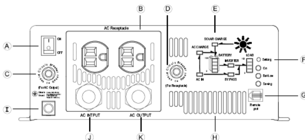
Figura 2 – Panel Frontal
