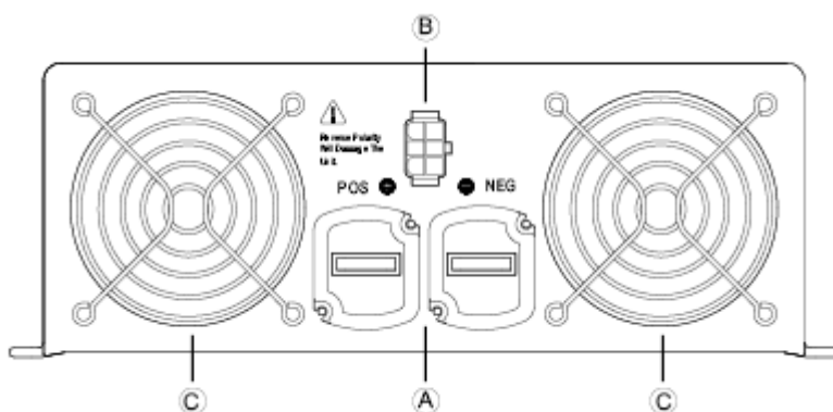
Figura 4 – Panel Trasero
