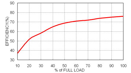
MKC03-48S05 Efficiency vs. Output Load
