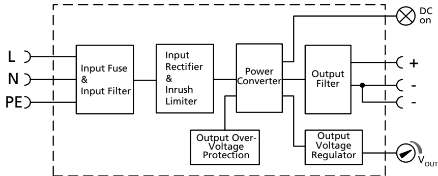
Fig. 9-1 Functional diagram
