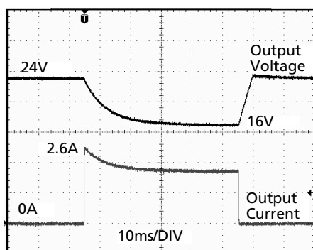
Fig. 22-1 Peak loading with 2x the nominal current for 50ms, typ.
