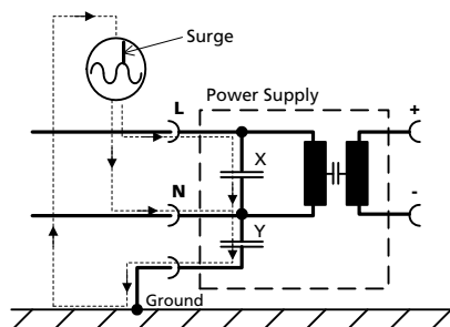
Fig. 22-3 Earthed input
