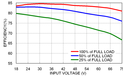
MOP03-48S05WA Efficiency vs. Input Voltage
