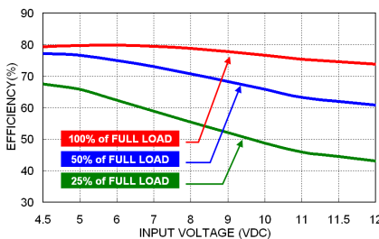
MPS(H)02-05S05 Efficiency vs. Input Voltage
