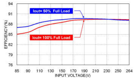
MSD30US24B Efficiency vs. Input Voltage
