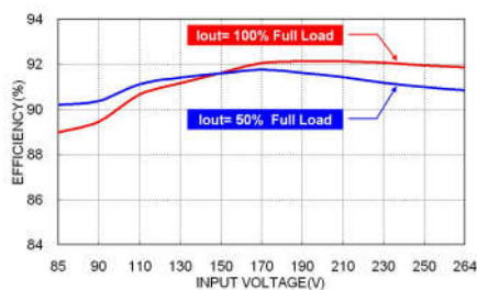
MSD40US24 Efficiency VS Input Voltage
