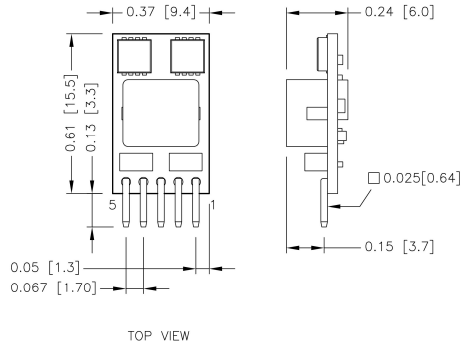
OSR03-05S2P5
