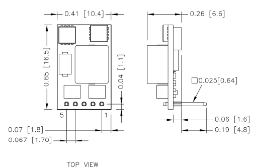
OSR03-24S05A/OSR03-24S12A
