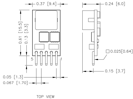
OSR03-24S05/OSR03-24S12
