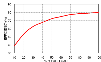
PDS03-48S05W Efficiency vs. Output Load
