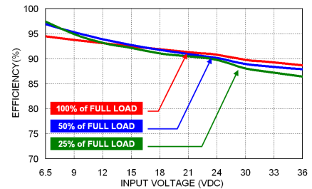
PSR02-12S05 Efficiency vs. Input Voltage
