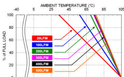
QAE100-48S05 Derating Curve With 0.24" Height Heat-sink
