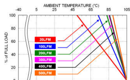
QAE100-48S05 Derating Curve With 0.5" Height Heat-sink
