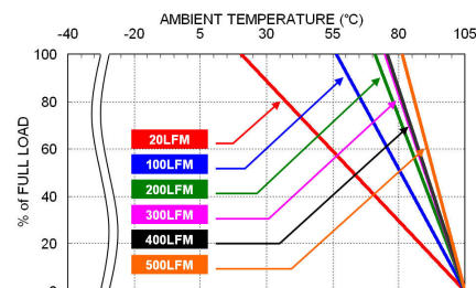
QAE150-24S05W Derating Curve With 0.5" Height Heat-sink
