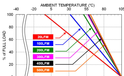
QAE150-24S05W Derating Curve With 0.24" Height Heat-sink
