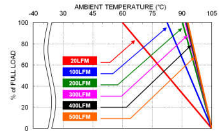
QAE60-72S05U Derating Curve With 0.5" Height Heat-sink (See Thermal Considerations)
