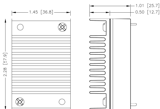
QAE60-□□S□□U - HS1 7G-0030B-F
