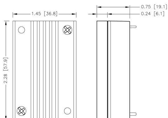
QAE60-□□S□□U - HS2 7G-0031B-F
