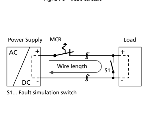
Fig. 24-5 Test circuit
