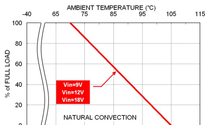
RCD15-12 Derating Curve
