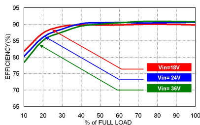
RCD15-24S05 Efficiency vs. Output Load
