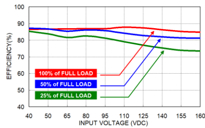
RDL10-110S12W Efficiency vs. Input Voltage
