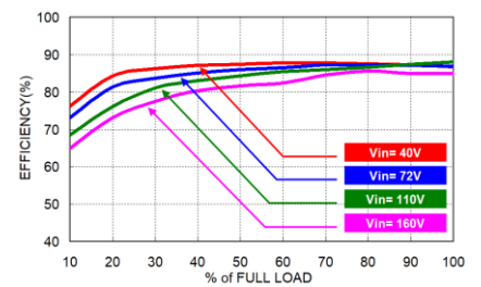
RDL10-110S12W Efficiency vs. Output Load
