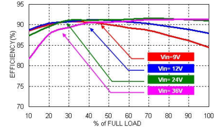
RED60-24S05W Efficiency vs. Output Load
