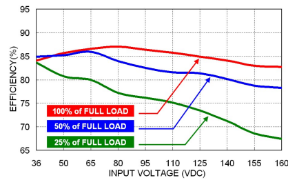
RHK10-110S05W Efficiency vs. Input Voltage
