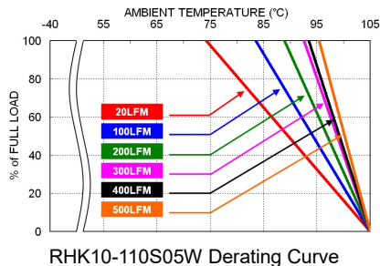
RHK10-110S05W Derating Curve
