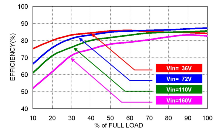
RHK10-110S05W Efficiency vs. Output Load
