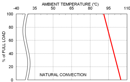
SDS(H)01-48S05W Derating Curve
