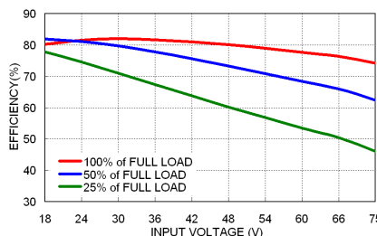
SDS(H)02-48S05W Efficiency vs. Input Voltage
