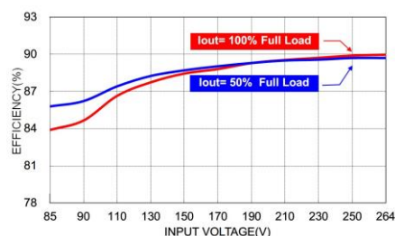
TAH240US24 Efficiency vs. Input Voltage
