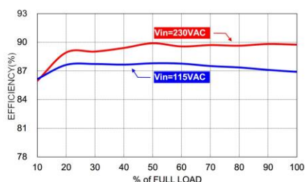
TAH240US24 Efficiency vs. Output Load
